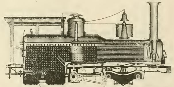
BALDWIN'S COAL BURNING BOILER FIG. 68
